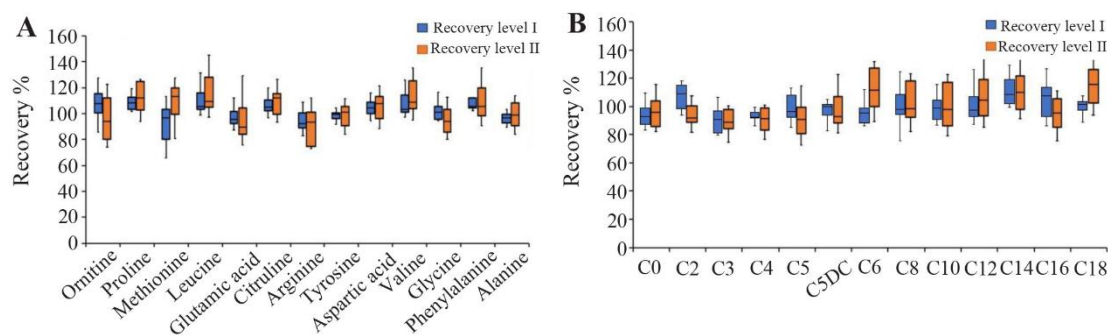
Figure 1. Box plots showing the recovery (%) of (A) amino acids and (B) acylcarnitines at levels I and II.
