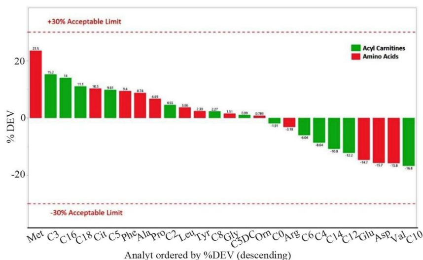
Figure 4. Deviation percentages for 40 real samples analyzed using PH NBS-D and MassChrom® kits (n=40).
