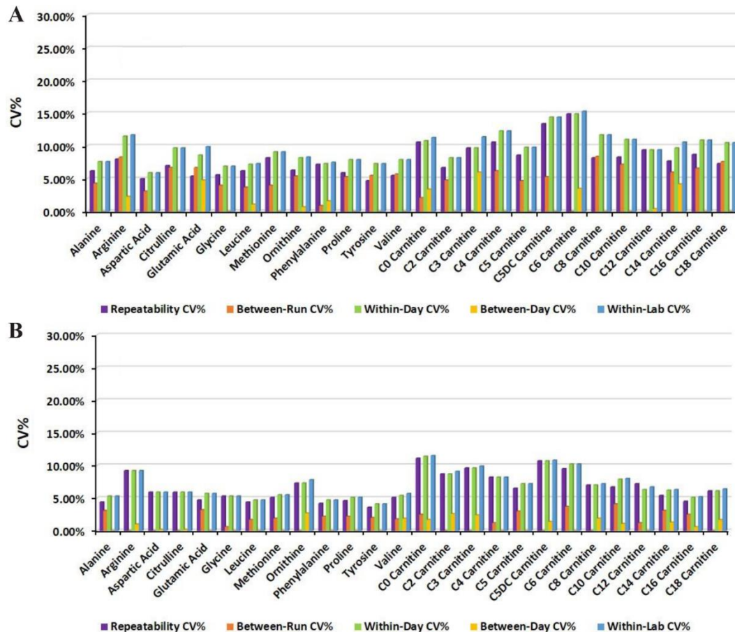
Figure 2. Intra-lab precision (%CV) of amino acids and acylcarnitines at a) level I and b) level II.
