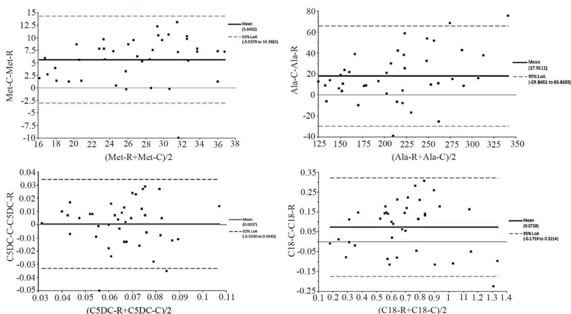
Figure 5. Bland–Altman plots of Met, Ala, C5DC and C18. R: Reference kit (MassChrom), C: Candid kit (PH NBS-D).
