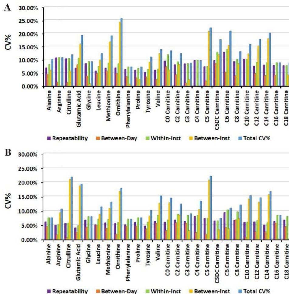
Figure 3. Interlaboratory precision (%CV) of amino acids and acylcarnitines at A) level I and B) level II.
