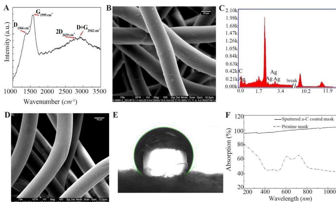
Figure 3. Properties of the SAC-Ag-coated surgical mask: A) Raman spectrum; B) SEM image of SAC-Ag-coated fibers; C) EDX spectrum; D) SEM image after bending and tape-adhesion tests; E) Water contact angle; and F) Optical absorption spectra of pristine and SAC-Ag-coated masks.
