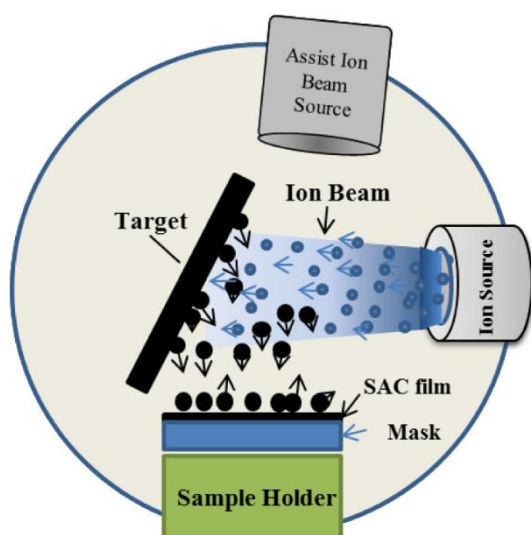
Figure 1. Schematic of IBSD system for SAC-Ag deposition.
