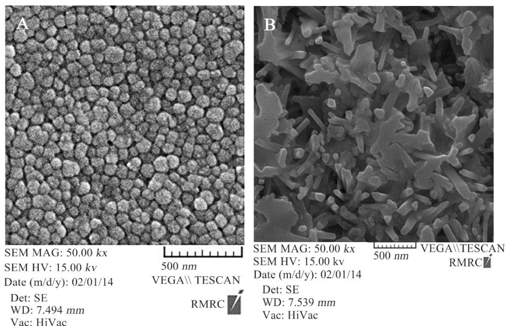
Figure 1. FESEM images of SeNPs, A) FESEM image of plain SeNPs showing the size of 60 nm. B) FESEM image of fabricated \text{CaSO}_4\text{@SeNPs} demonstrating nanocomposites are rod shaped (400×100 nm).
