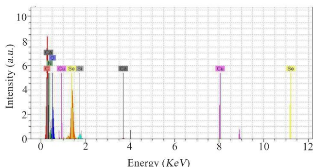
Figure 3. The illustration shows the presence of Se atoms and the existence of elemental NPs in the EDS spectrum of \text{CaSO}_4\text{@SeNPs} . Additional peaks of copper, carbon, oxygen, and nitrogen elements are attributed to the grid used for FESEM imaging or calcium compound.
