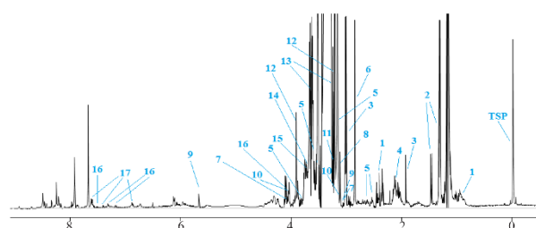
Figure 5. The representative 400 MHz CPMG ^1\text{H} -NMR spectrum of rat stomach tissue. Altered metabolites between normal and indomethacin-induced gastric ulcer samples are demonstrated. Key: 1-pantothenate, 2-isoleucine, 3-spermidine, 4-methionine, 5-acetylcarnitine, 6-trimethylamine, 7-creatinine, 8-carnitine, 9-cis-aconitate, 10-choline, 11-aurine, 12-betaine, 13-glucose, 14-N,N-Dimethylglycine, 15-acetylcholine, 16-tryptophan, 17-kynurenine.
